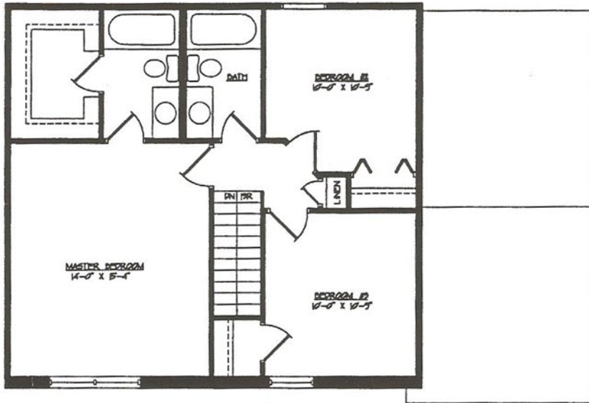
SECOND FLOOR LEVEL PLAN 706 SQFT.
